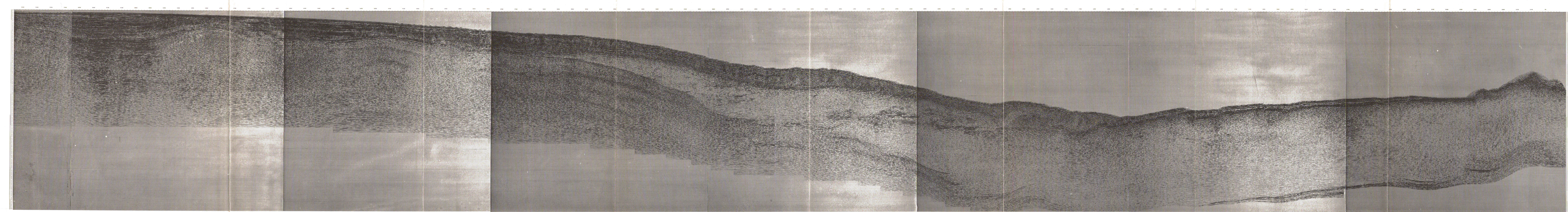
Figure 4 Multichannel seismic reflection profile of migrated record section off Joban District , Northeast-Japan abscissa: 500 meters/division, ordinate: 0.1 seconds/division (two-way) vertical exaggeration : 2.5 (at sea bottom)
